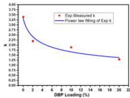
Dielectric Constant of PPI variation with porogen concentration
