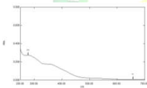
Figure 1: UV-vis spectroscopy of chitosan nanocomposite of cobalt oxides
