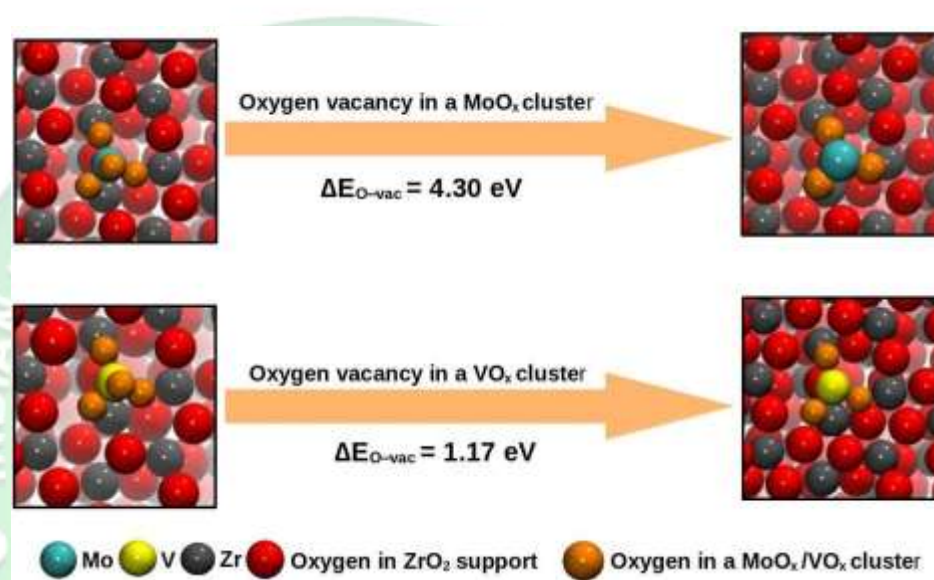
Figure 1. Top views of optimized structure of isolated monomeric clusters of MoO x and VO x supported on on ZrO 2 . The figure on the right panel shows the optimized structure of clusters after the creation of an oxygen vacancy.
