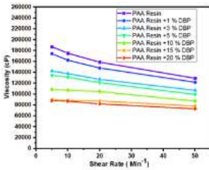
Viscosity of PAA resin & Mixed Resin variation with shear rate
