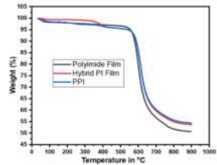
Thermal stability of polyimide film, hybrid PI film and PPI
